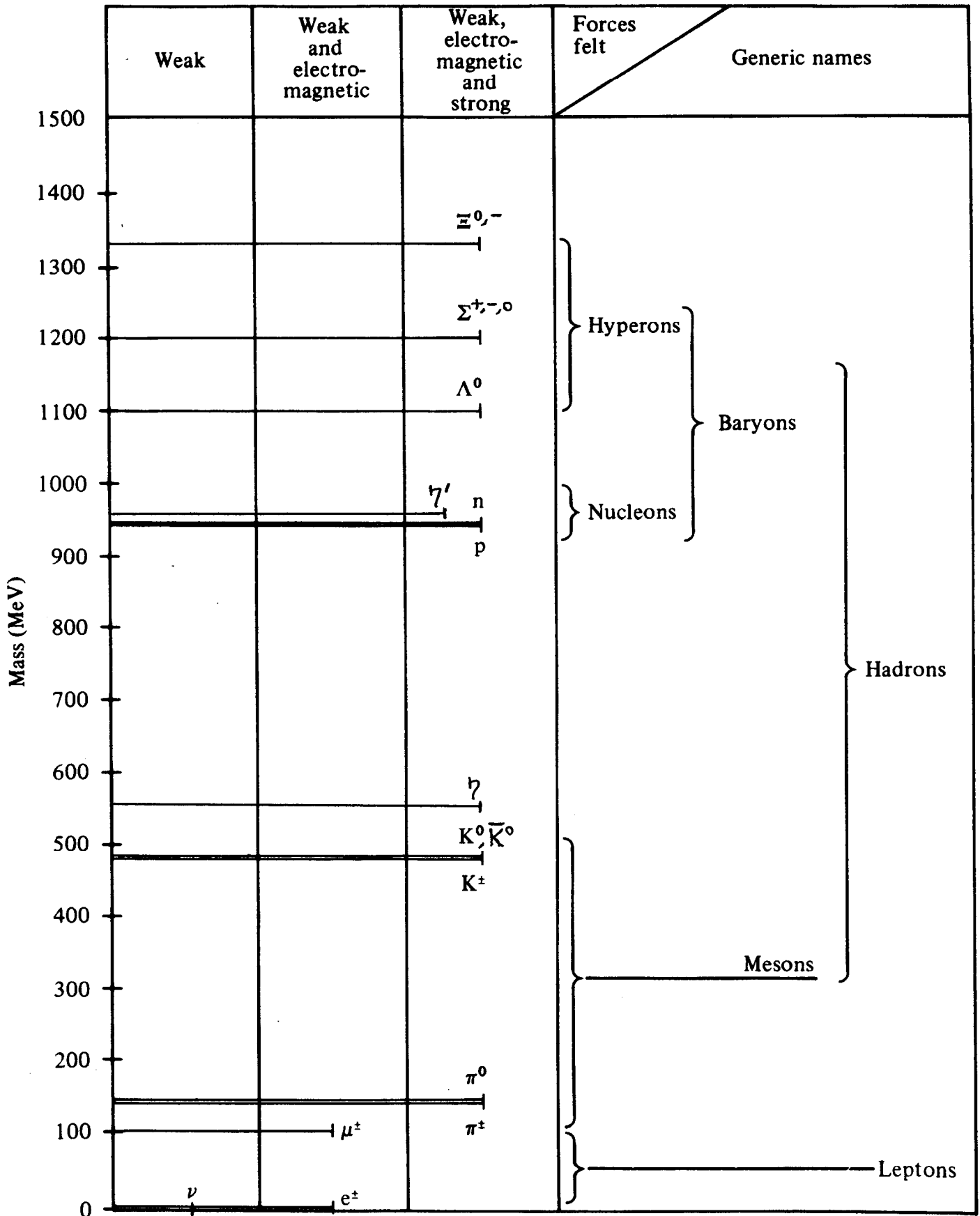
Fig. 8.4. The basic set of elementary particles known by the early 1950s.
